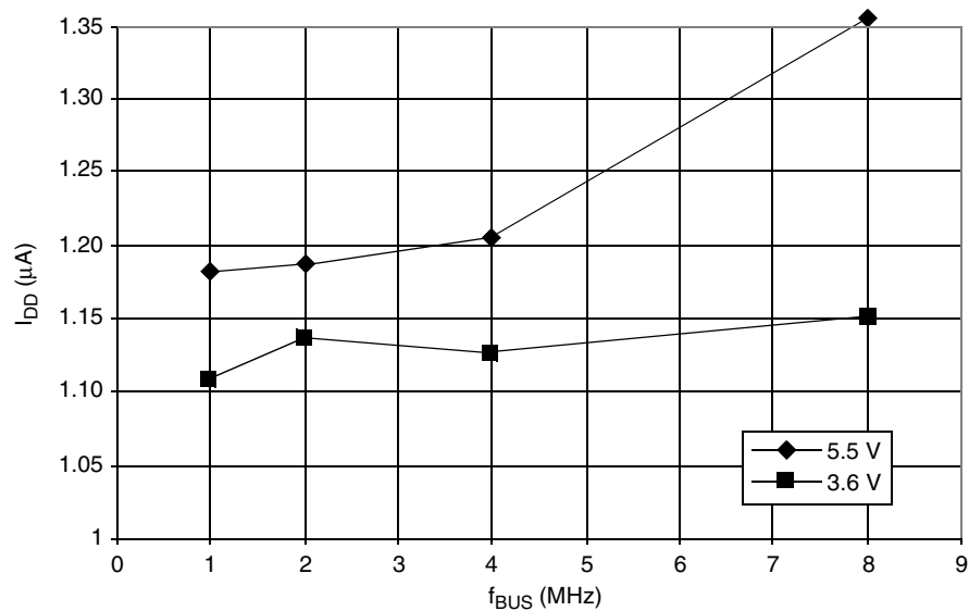
Figure 23-15. Typical Stop Mode I_{\text{DD}} , with all Modules Disabled ( -40\text{ }^{\circ}\text{C} to 85\text{ }^{\circ}\text{C} )
